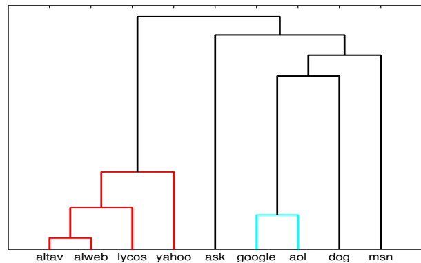
Figure 7: Hierarchical clustering dendrogram for the nine search engines over the query category Companies.
