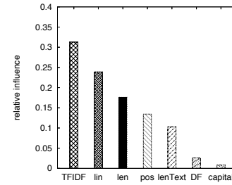
Figure 1: The relative influence of each feature in GBM
