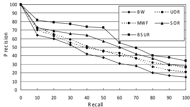
Figure 7. Precision at 11 Standard Recall Levels
