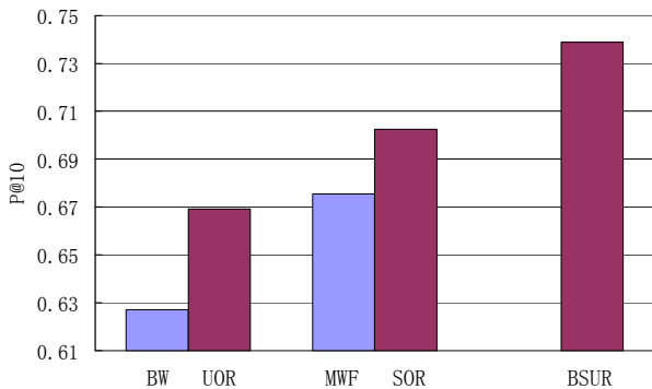
Figure 4. Precision at 10
