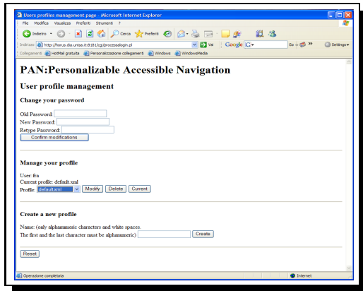
Figure 2: Users's Profile Management.
